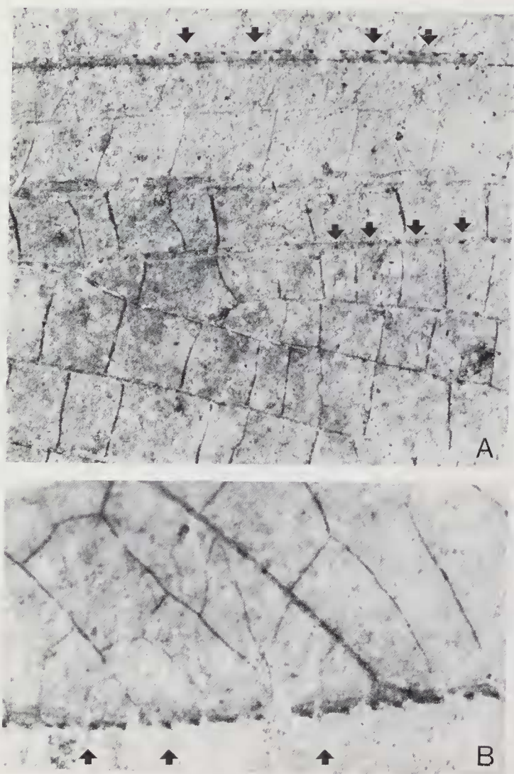
Figure 5. Protoreisma latum Sellards. Photographs of neotype, MCZ 3419a, from Permian of Kansas, showing A, anterior part of hind wing, the arrows pointing to setal bases along the front margin of the wing and on certain veins ( \times 24 ); B, posterior part of same wing, the arrows pointing to the serrated hind margin ( \times 38 ).
